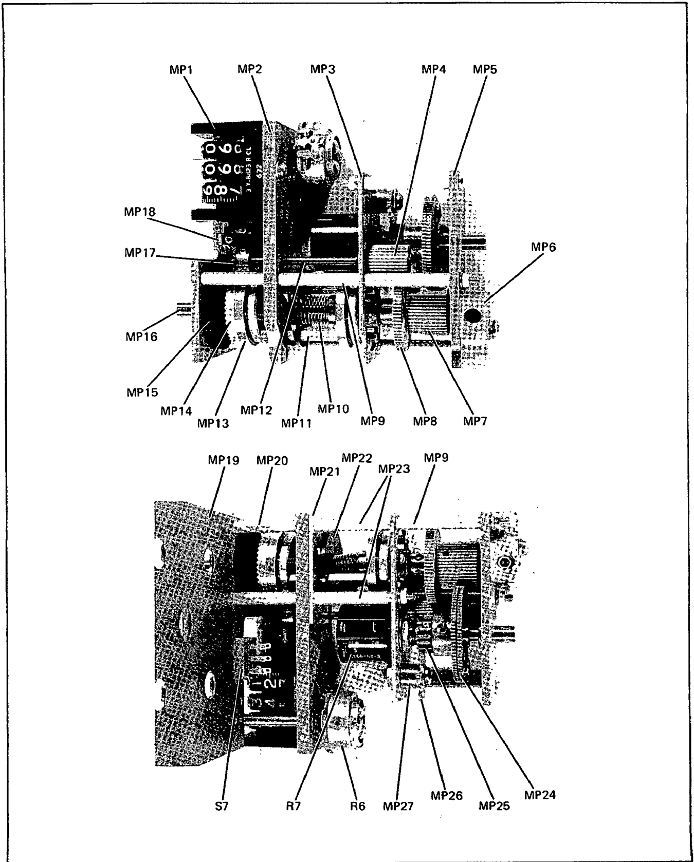
Figure 6-1. Frequency Control Component Locator.
