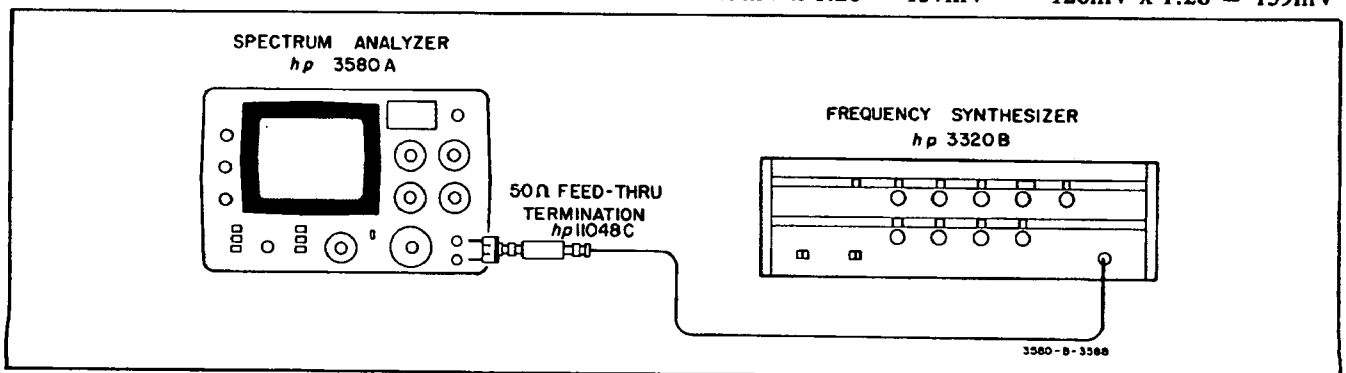
Figure 5-6. Proper Hookup.
