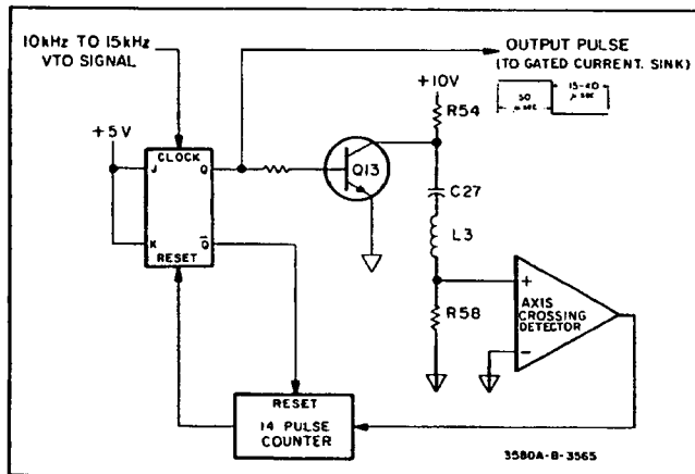
Figure 4-16. Precision Monostable.
