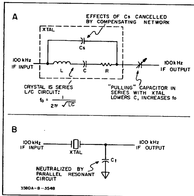
Figure 4-3. Crystal Filter.
