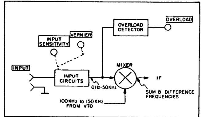
Figure 3-7. Input Section.
