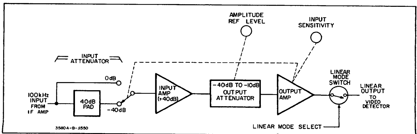
Figure 4-5. Linear Amplifier.
