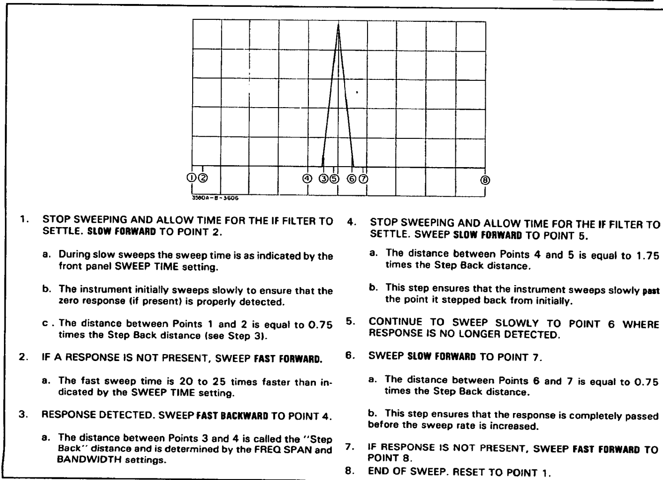
Figure 4-11. Adaptive Sweep Routine.
