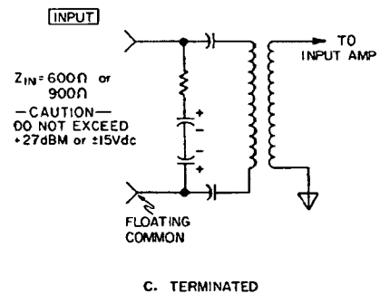
Figure 8-1. Balanced-Terminated Input Configuration.
