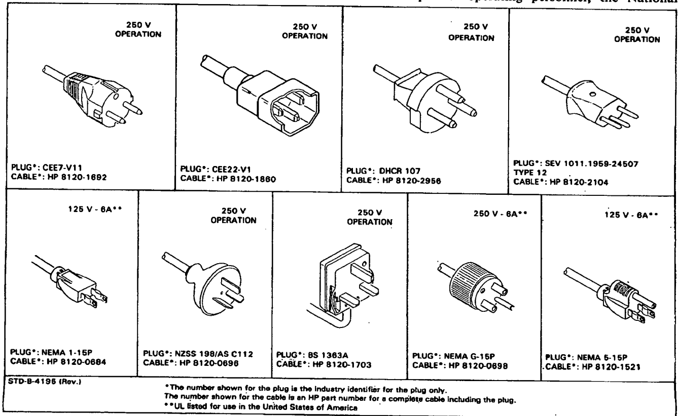
Figure 2-1. Power Receptacles.
